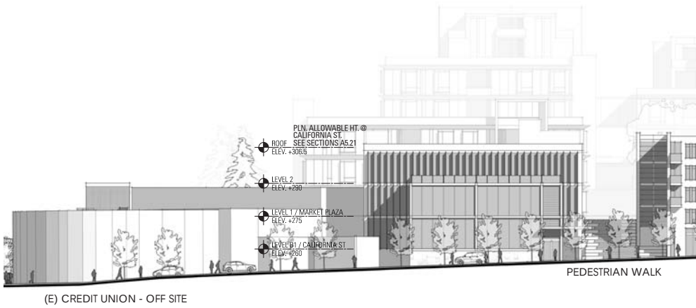
1. CALIFORNIA STREET ELEVATION (NORTH)
